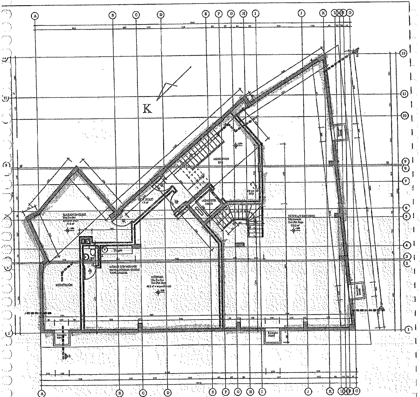
BODRUM KAT PLANI 1/50
